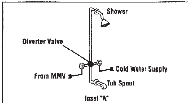
Typical ASSE 1016 installation*
