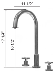
CENTER TO CENTER 10 1/2"
